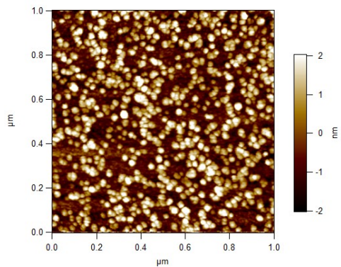
Figure 1. AFM image showing a rutile TiO 2 (110) crystal surface sensitized with CdSe quantum dots after 200 cycles of the ALD TiO 2 grown via tetrakis(dimethylamido)titanium (IV)/H 2 O at 150°C.
