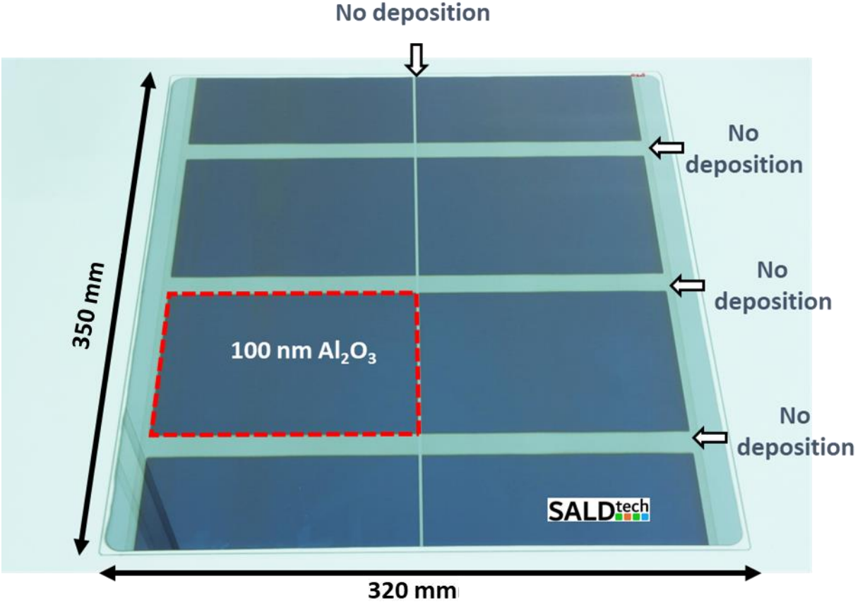
Fig. 1: Mask-less patterned Spatial ALD of 100 nm Al 2 O 3 on a 320 mm x 350 mm glass plate. The glass plate was metallized prior to deposition for visualization of the Al 2 O 3 layer through interference.
