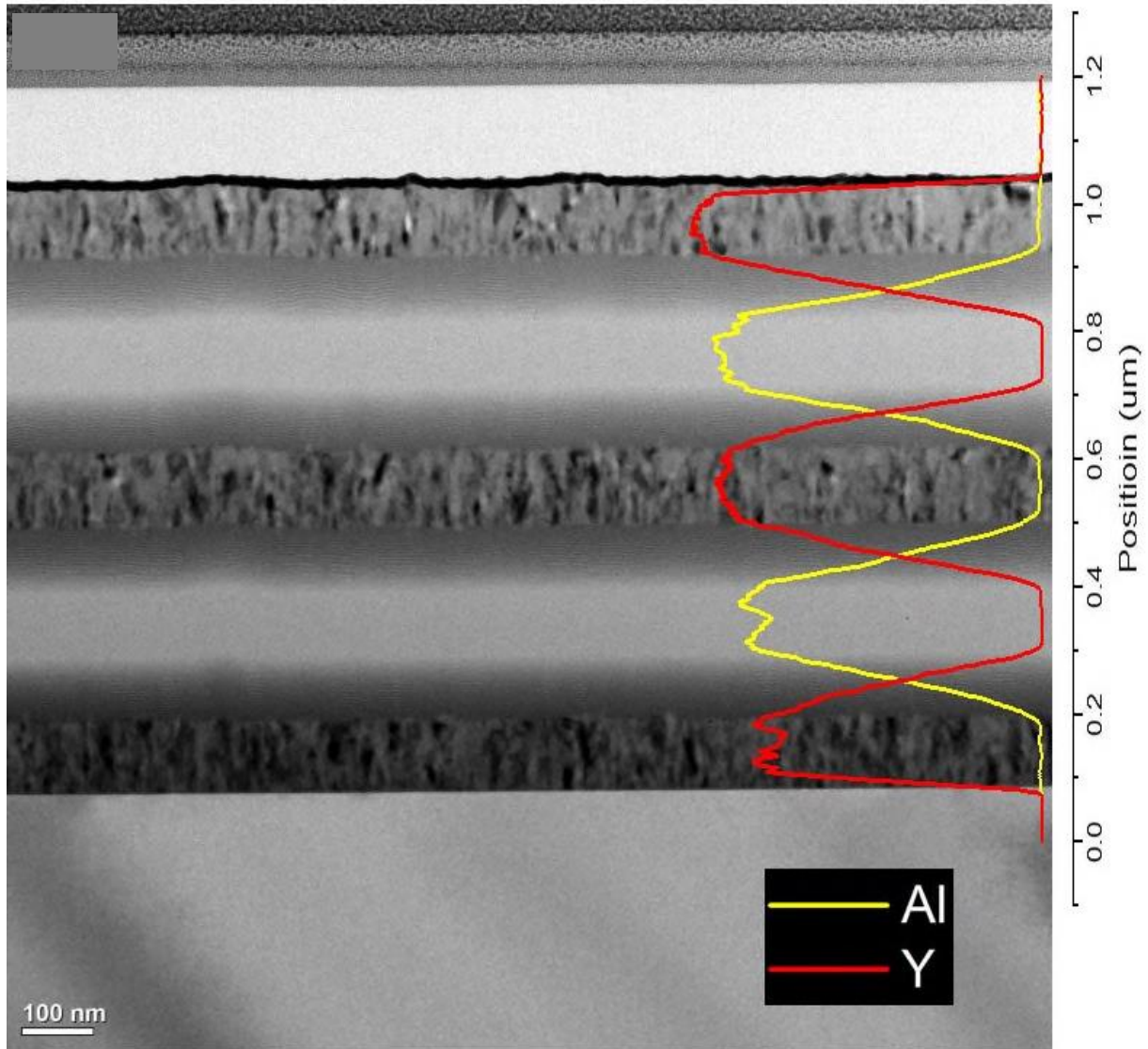
Figure 1: TEM cross section of compositionally graded laminate transitions between alternating Y_2O_3 and Al_2O_3 layers with EDS line scan overlaid.
