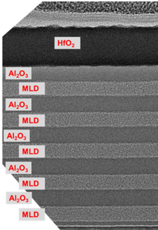
Fig. 1: TEM-picture of an ALD/MLD nanolaminate
