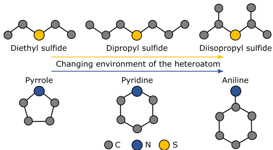
Fig. 1. Schematic illustration showing the investigated small molecule inhibitors with their unique alignment of the heteroatom.
