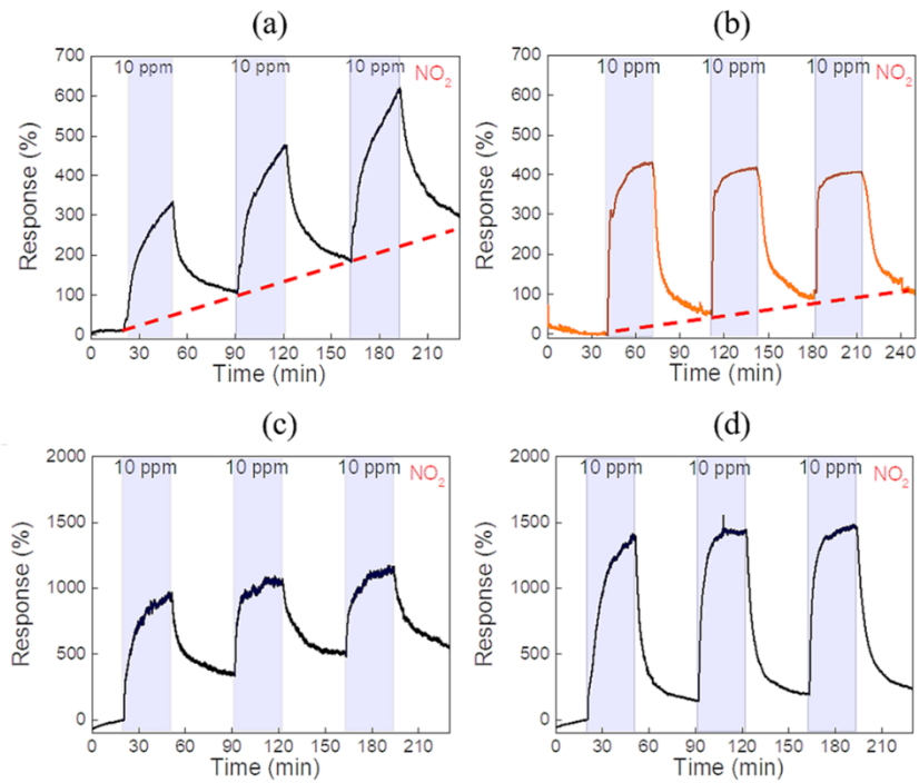
Figure 2. \text{NO}_2 sensing characteristics of (a) pristine \text{MoS}_2 , (b) selectively passivated \text{MoS}_2 , (c) pristine \text{WS}_2 , (d) selectively passivated \text{WS}_2
