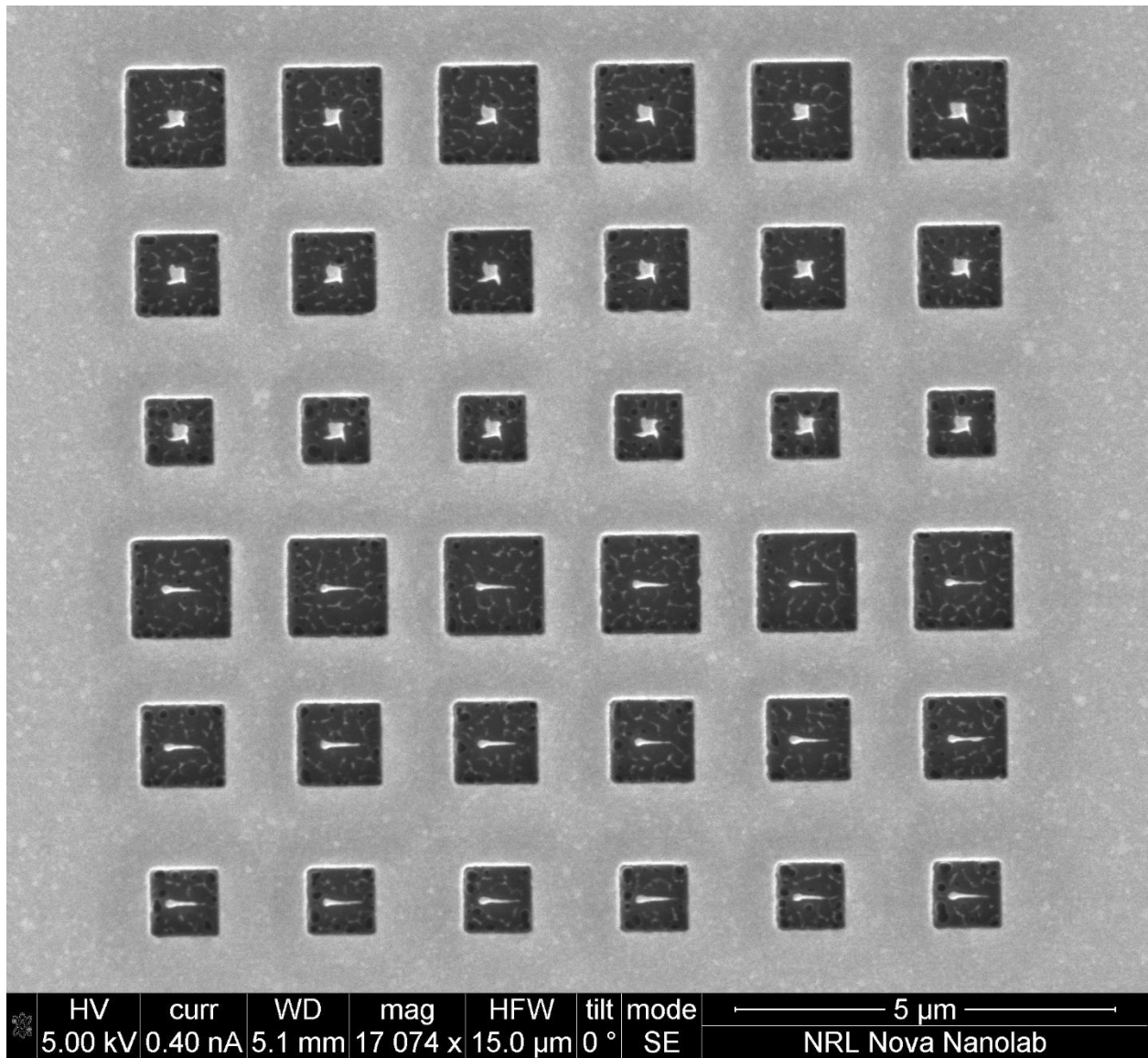
Figure 1. SEM image of an array of plasmonic nanoparticles patterned by FIB milling of 25nm Au layer sputtered on 100nm thick ZEP520A copolymer on a Si substrate.
