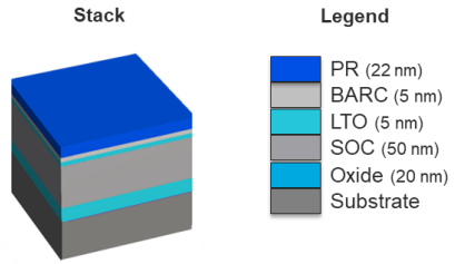
Fig. 1: Example blanket patterning stack for PR evaluation
