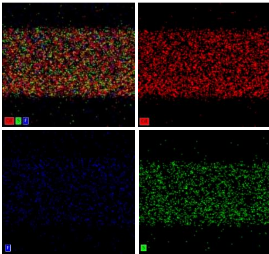
Figure 1. TEM–EDS elemental mapping images of Cadmium (Cd), Sulfur (S), and Fluorine (F) in the CdS–PPFC nanocomposite thin film.
