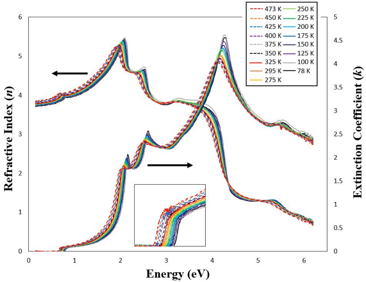
Fig. 1 – Refractive Index and Extinction Coefficient for a GaSb wafer for temperatures ranging from 78 – 473.2 K. Insert shows the extinction coefficient at the absorption band edge.
